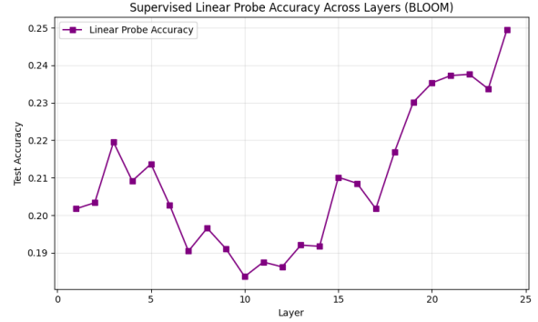
Figure 7: Supervised linear probe accuracy across layers for BLOOM. Accuracy ranges from 0.19 to 0.25.
