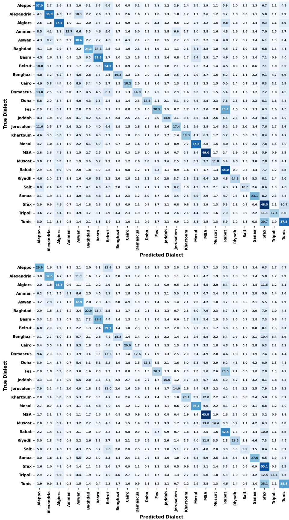
Figure 10: Complete dialectal confusion matrices for mGPT (top) and BLOOM (bottom).
