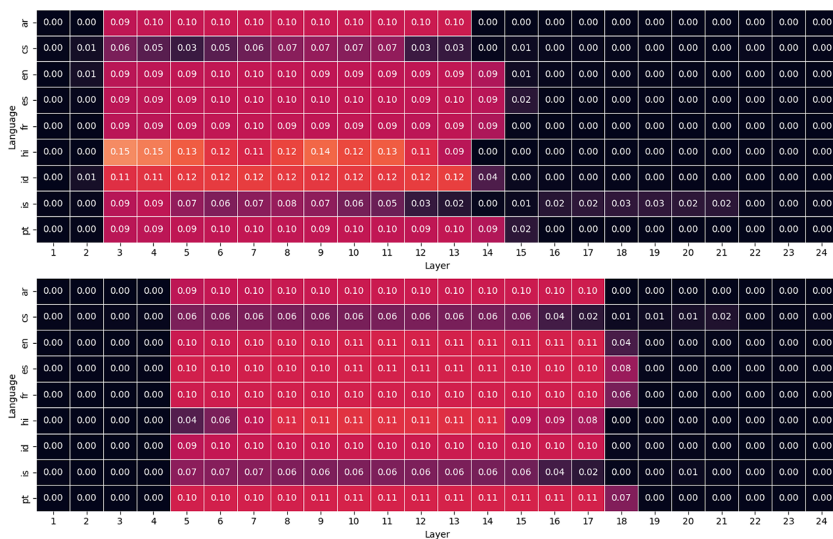
Figure 13: Replicated layer-wise dominance scores for mGPT (top) and BLOOM (bottom).
