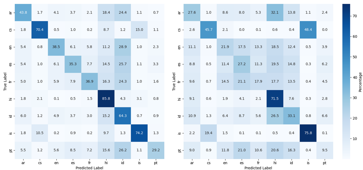
Figure 12: Replicated confusion matrices for mGPT (left) and BLOOM (right).
