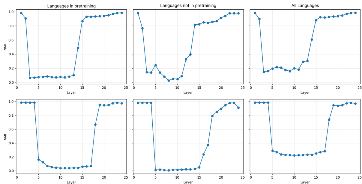
Figure 11: Replicated NMI curves for mGPT (top) and BLOOM (bottom).
