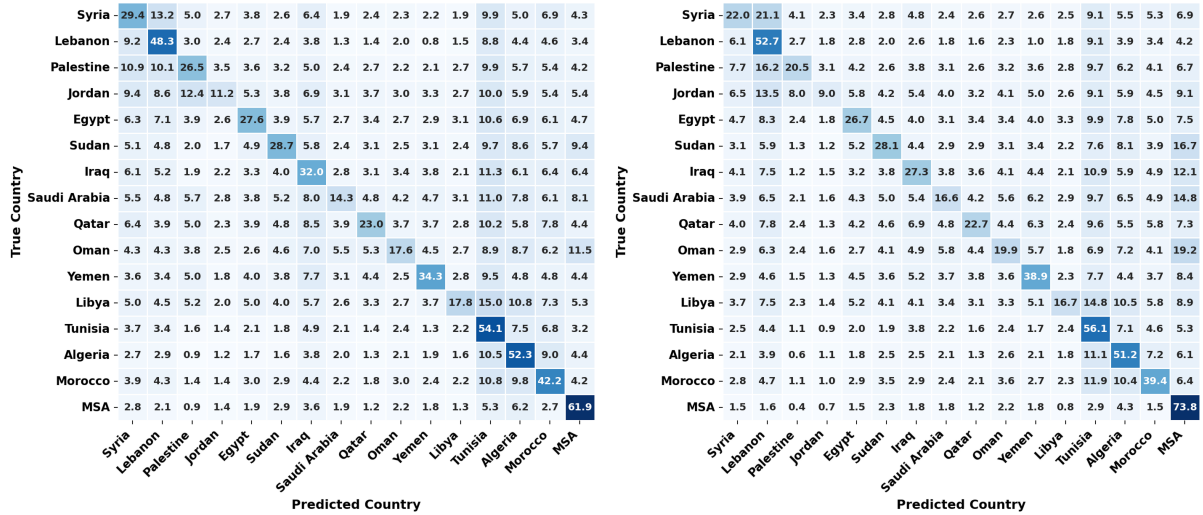
Figure 2: Confusion matrices for dialect clustering in mGPT (left) and BLOOM (right) grouped by country. Clear diagonals show that dialect identity is preserved despite low separability.
