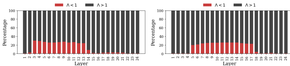
Figure 14: Replicated token-level dominance statistics for mGPT (left) and BLOOM (right).
