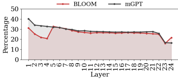
Figure 3: Token-level dominance statistics. Percentage of tokens with \Lambda < 1 . A mostly flatline percentage of tokens are being assigned to competing dialects.
