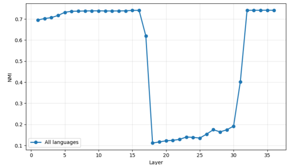
Figure 6: Layer-wise NMI values for ArabianGPT-08B-V2. Dialect separability remains high until later layers before collapsing sharply.
