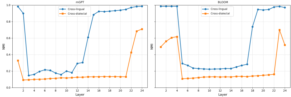
Figure 1: Layer-wise NMI values for cross-lingual vs. cross-dialectal representations for mGPT (left) and BLOOM (right). Dialectal NMI is lower and remains low over a wider middle-layer range. Cross-lingual representations were computed using Parallel Universal Dependencies (PUD) treebanks (Zeman et al., 2017) (following Shani and Basirat (2025)), cross-dialectal representations were computed using the MADAR corpus (Bouamor et al., 2018).
