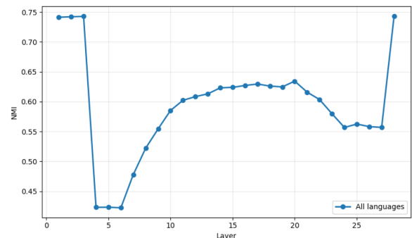
Figure 5: Layer-wise NMI values for Qwen2.5-7B. NMI drops sharply in early layers and partially recovers later.
