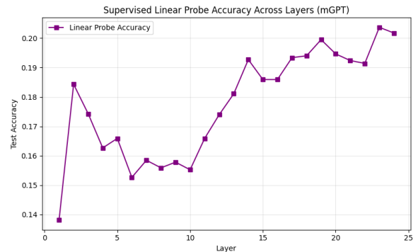
Figure 8: Supervised linear probe accuracy across layers for mGPT. Accuracy ranges from 0.14 to 0.21.
