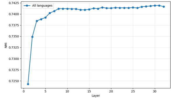
Figure 4: Layer-wise NMI values for Meta-Llama-3.1-8B-Instruct. The model maintains relatively stable dialect separability across middle and later layers.
