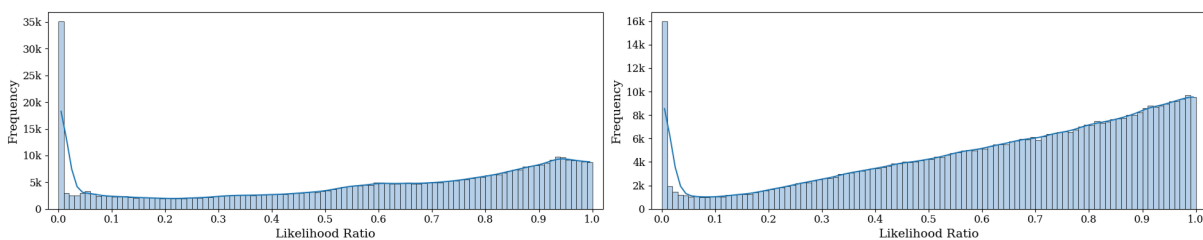
Figure 15: Replicated token-level \Lambda histograms for mGPT (left) and BLOOM (right).
